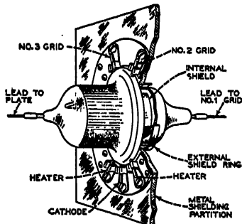
Typical shielding arrangement for a uhf vacuum tube.
